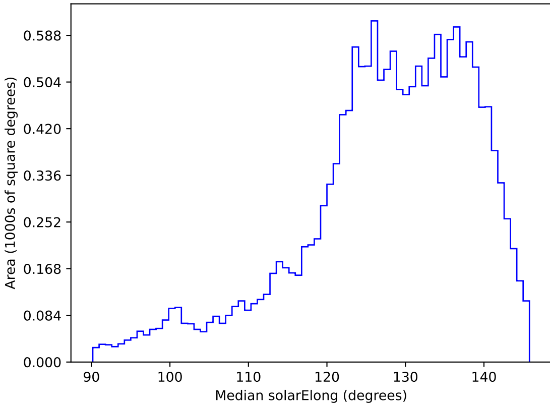
too_elab_r16_d2_gz_v3.4_10yrs WFD z band: Median solarElong
