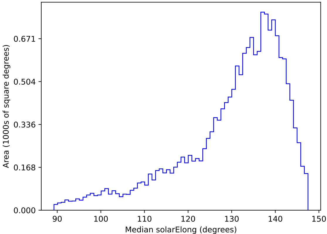
too_elab_r16_d2_gz_v3.4_10yrs WFD y band: Median solarElong
