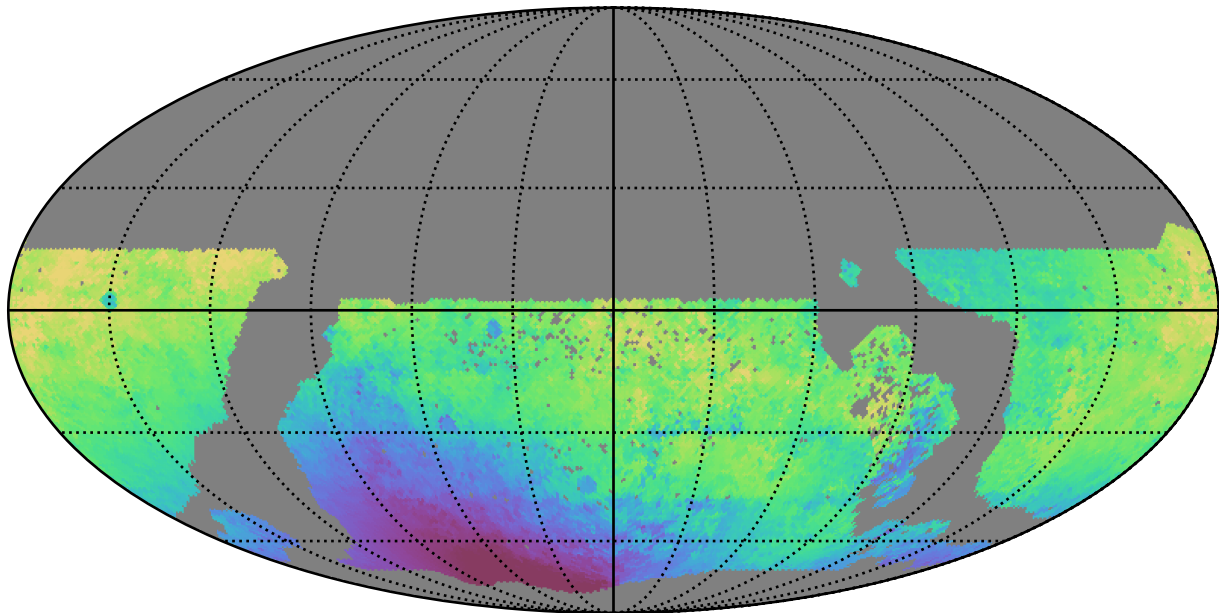
too_elab_r16_d2_gz_v3.4_10yrs WFD u band: Median solarElong
