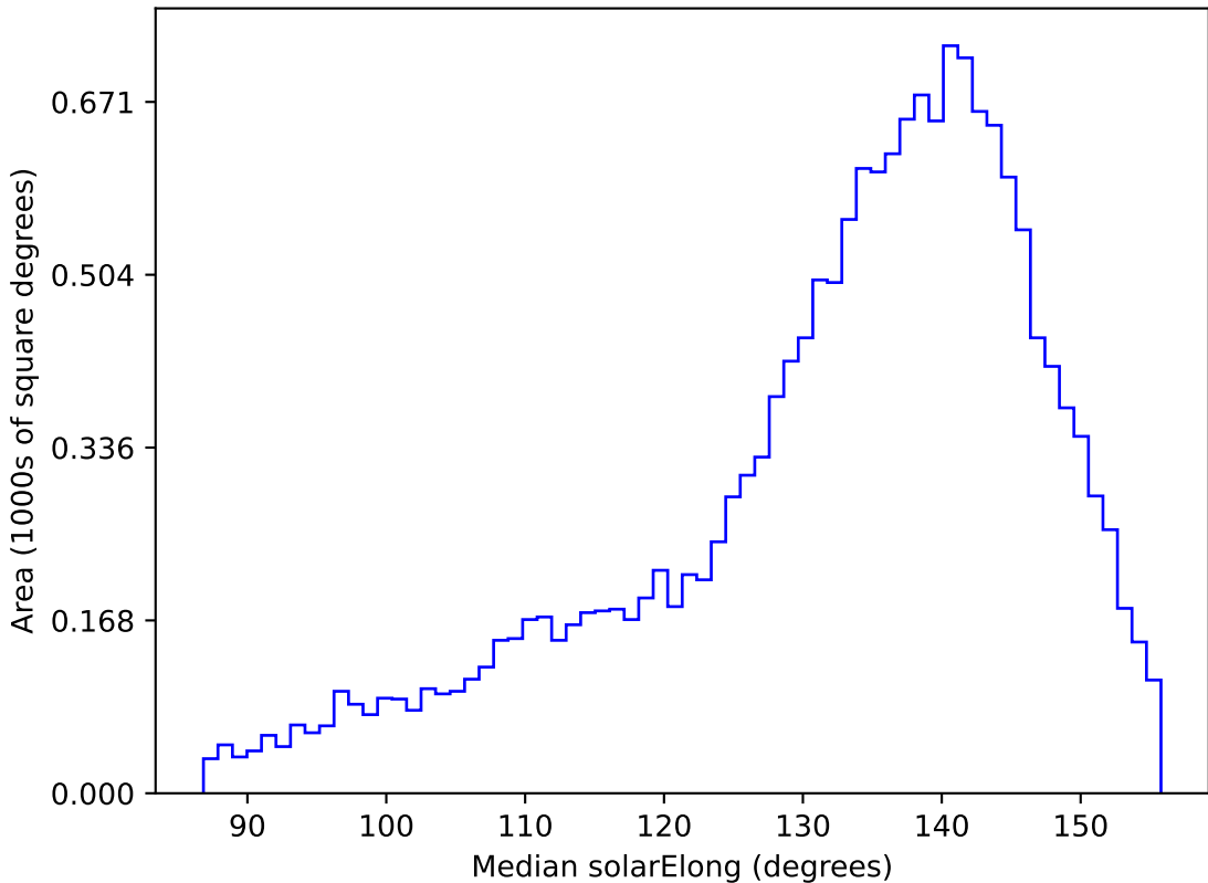
too_elab_r16_d2_gz_v3.4_10yrs WFD u band: Median solarElong
