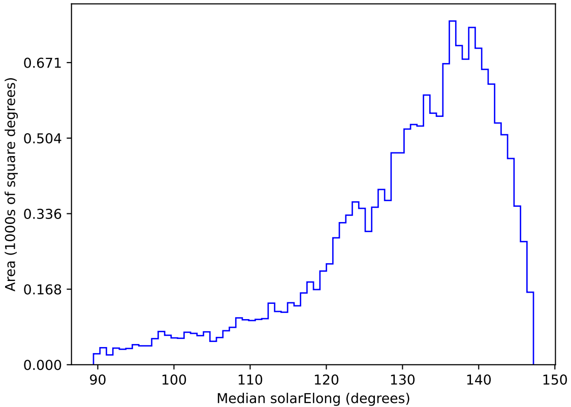
too_elab_r16_d2_gz_v3.4_10yrs WFD r band: Median solarElong
