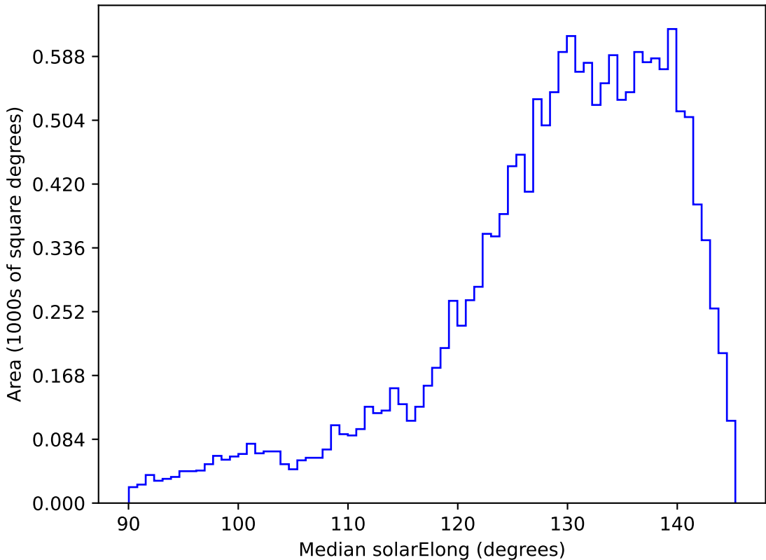
too_elab_r16_d2_gz_v3.4_10yrs WFD i band: Median solarElong
