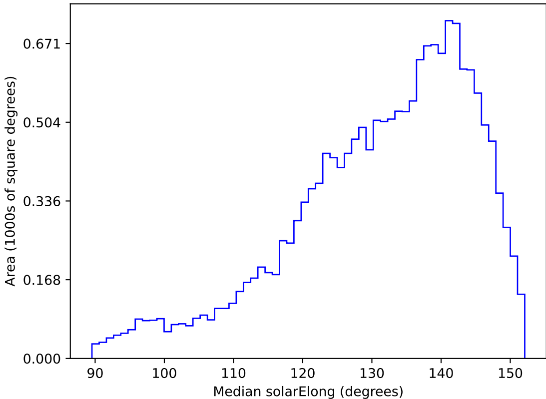
too_elab_r16_d2_gz_v3.4_10yrs WFD g band: Median solarElong
