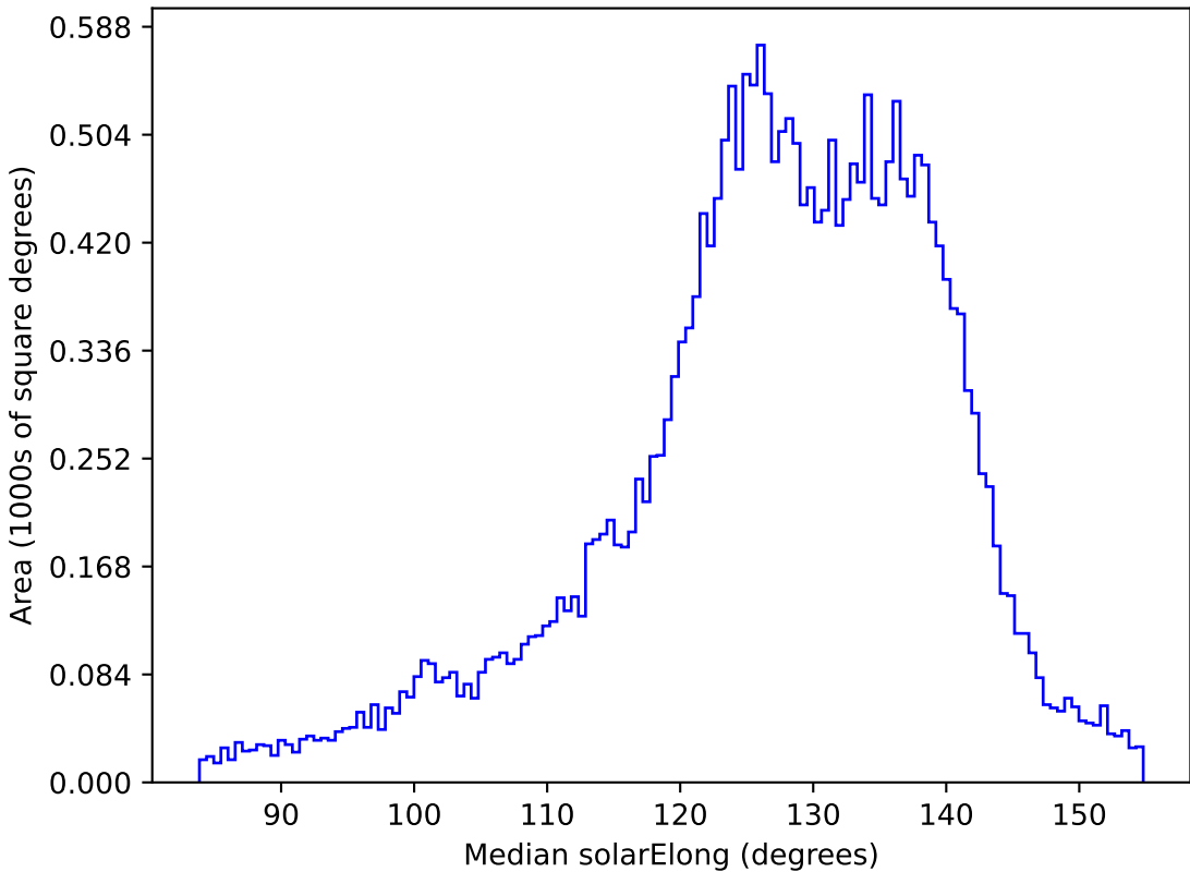
too_elab_r16_d2_gz_v3.4_10yrs All sky z band: Median solarElong
