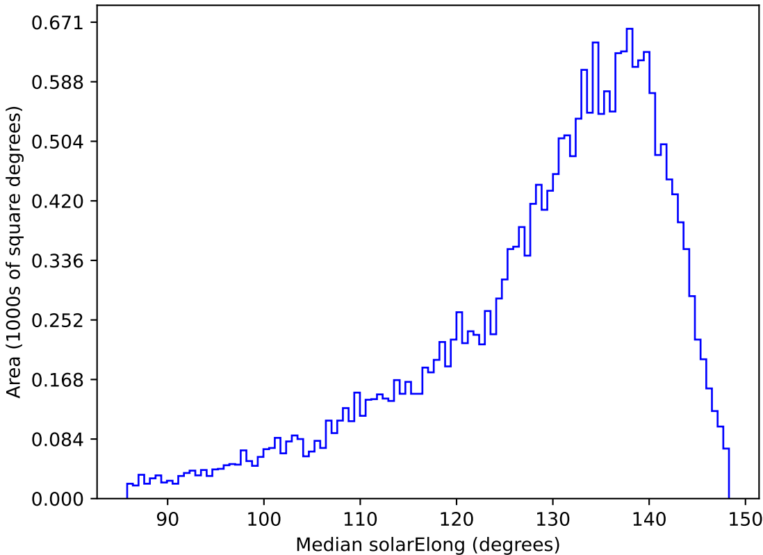
too_elab_r16_d2_gz_v3.4_10yrs All sky y band: Median solarElong
