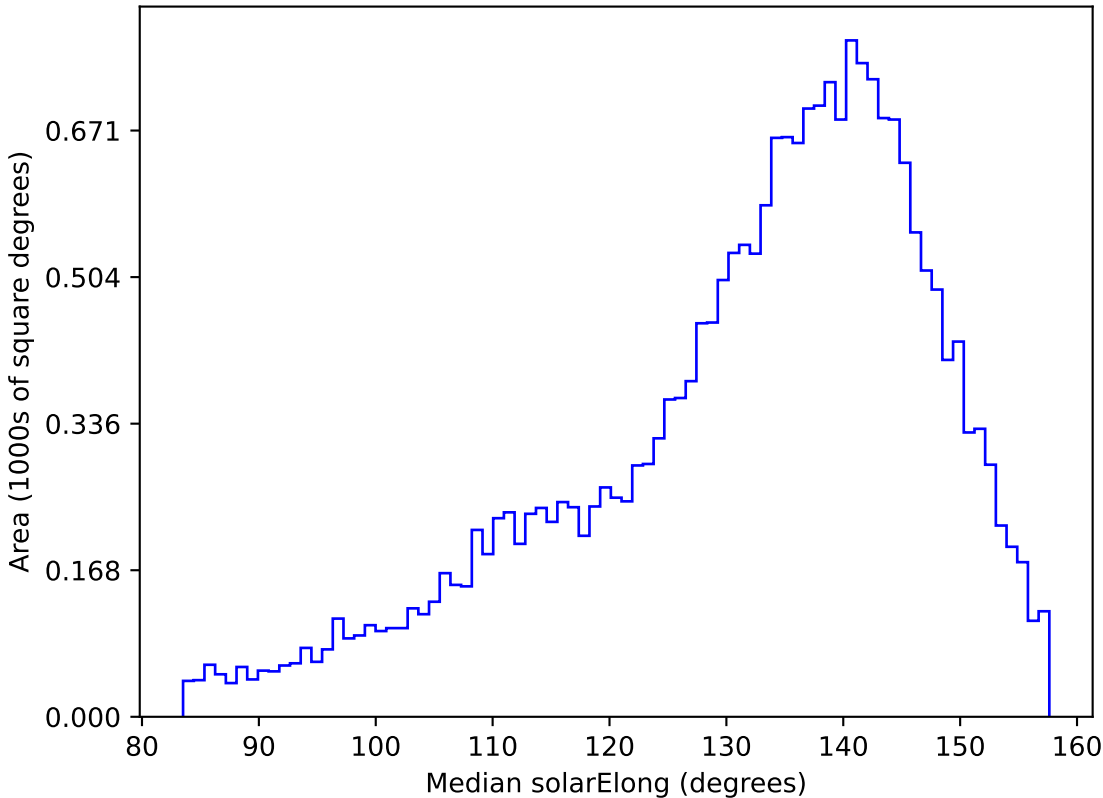
too_elab_r16_d2_gz_v3.4_10yrs All sky u band: Median solarElong
