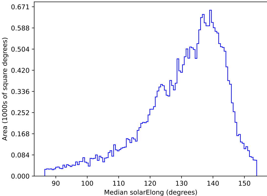
too_elab_r16_d2_gz_v3.4_10yrs All sky r band: Median solarElong
