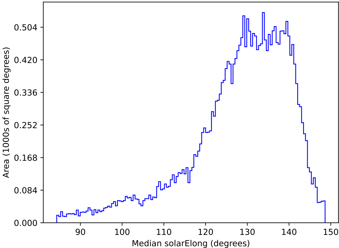
too_elab_r16_d2_gz_v3.4_10yrs All sky i band: Median solarElong
