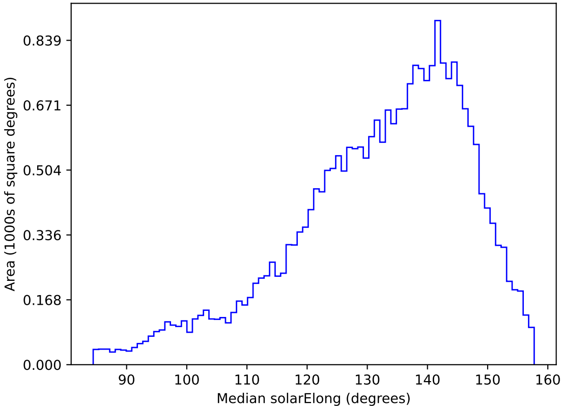
too_elab_r16_d2_gz_v3.4_10yrs All sky g band: Median solarElong
