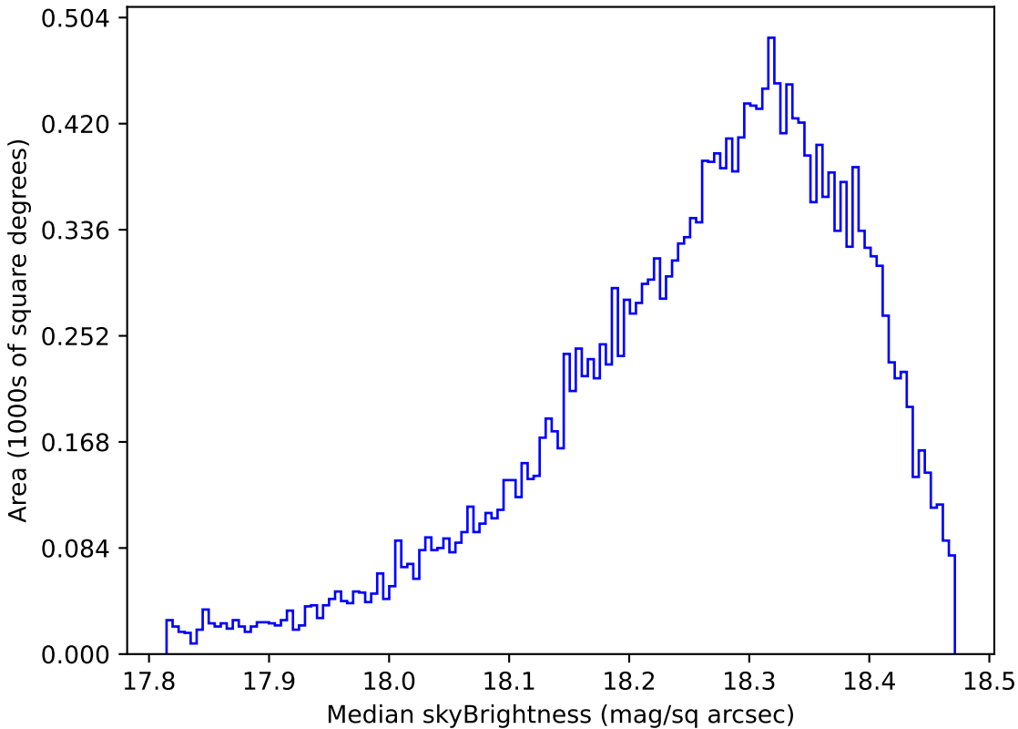
too_elab_r16_d2_gz_v3.4_10yrs Yr 1 y band: Median skyBrightness
