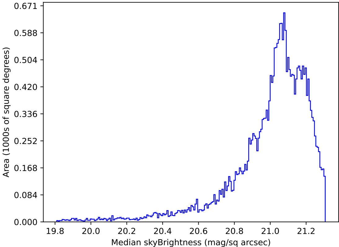
too_elab_r16_d2_gz_v3.4_10yrs Yr 1 r band: Median skyBrightness
