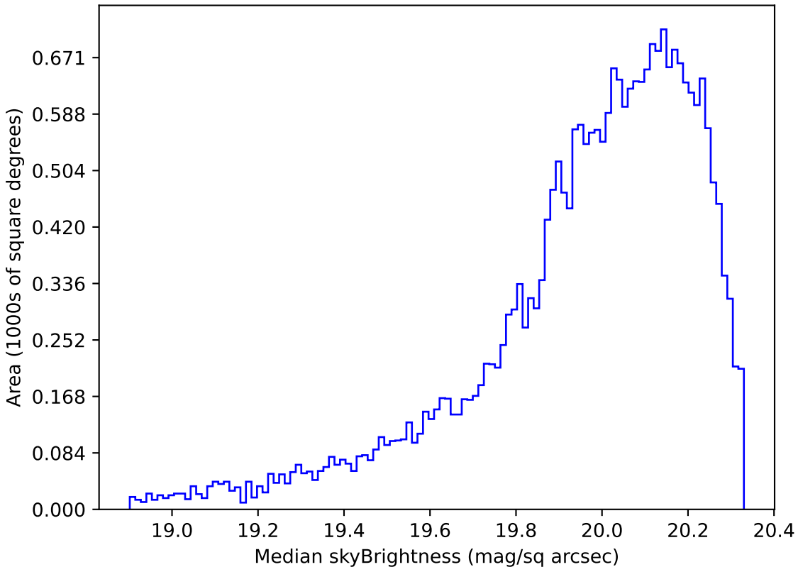
too_elab_r16_d2_gz_v3.4_10yrs Yr 1 i band: Median skyBrightness
