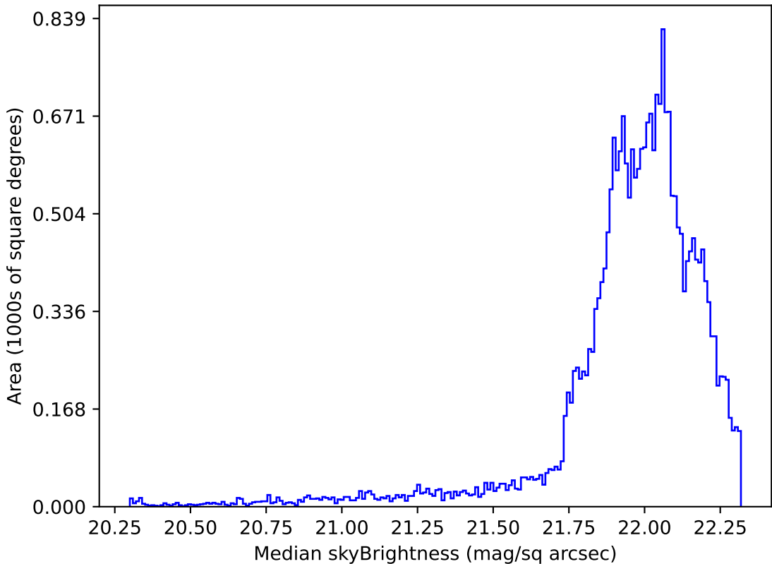
too_elab_r16_d2_gz_v3.4_10yrs Yr 1 g band: Median skyBrightness
