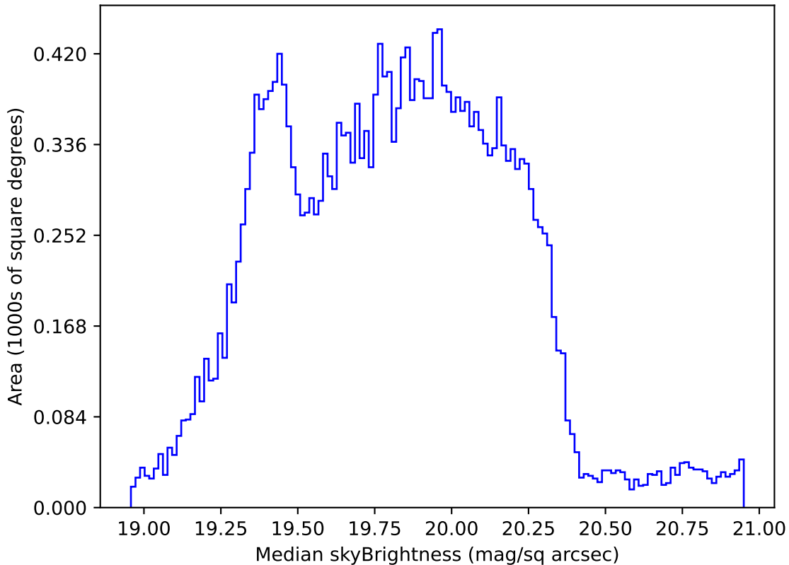
too_elab_r16_d2_gz_v3.4_10yrs Yr 1 all bands: Median skyBrightness
