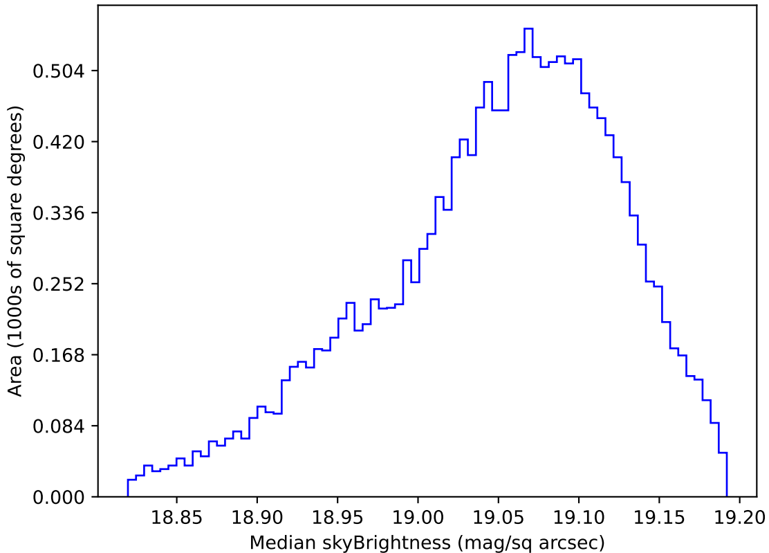
too_elab_r16_d2_gz_v3.4_10yrs WFD z band: Median skyBrightness
