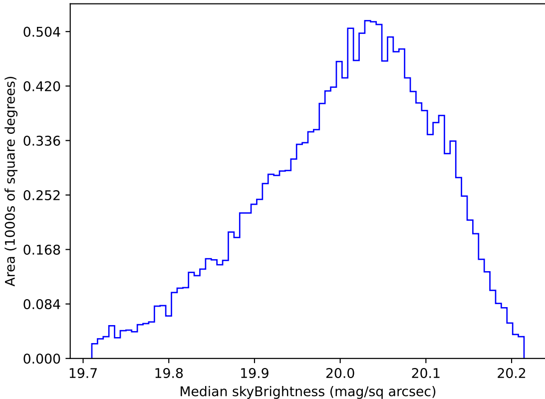
too_elab_r16_d2_gz_v3.4_10yrs WFD i band: Median skyBrightness
