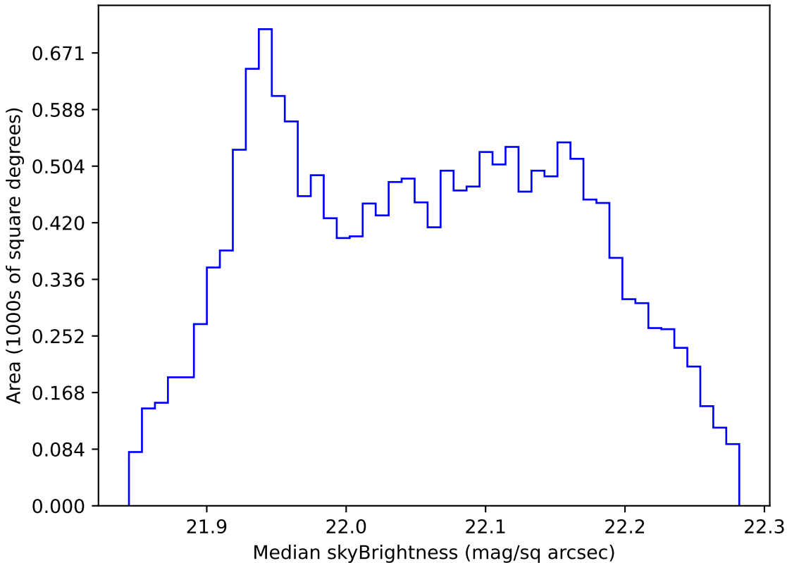
too_elab_r16_d2_gz_v3.4_10yrs WFD g band: Median skyBrightness
