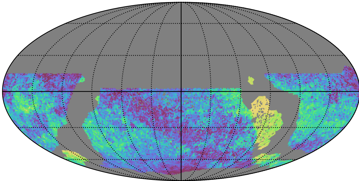
too_elab_r16_d2_gz_v3.4_10yrs WFD all bands: Median skyBrightness
