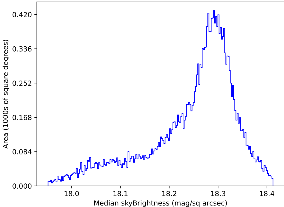
too_elab_r16_d2_gz_v3.4_10yrs All sky y band: Median skyBrightness
