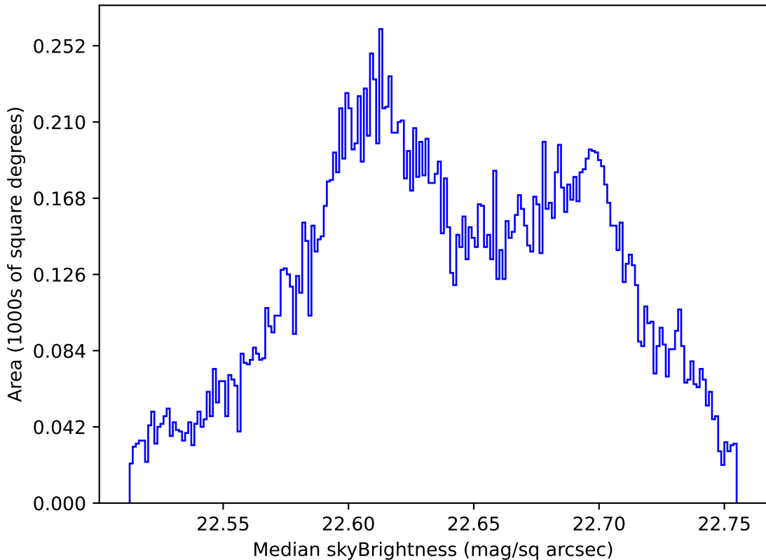
too_elab_r16_d2_gz_v3.4_10yrs All sky u band: Median skyBrightness
