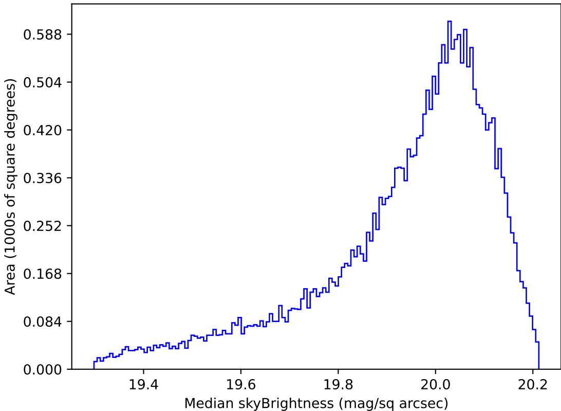
too_elab_r16_d2_gz_v3.4_10yrs All sky i band: Median skyBrightness
