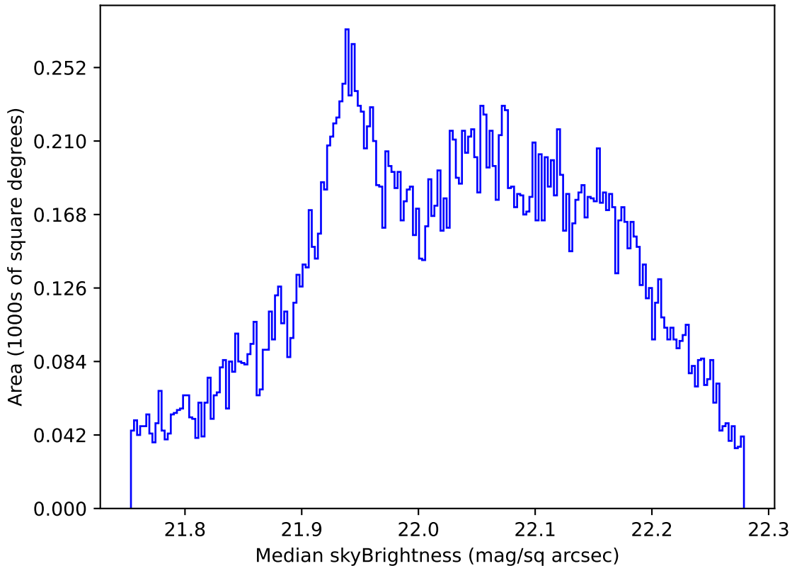
too_elab_r16_d2_gz_v3.4_10yrs All sky g band: Median skyBrightness
