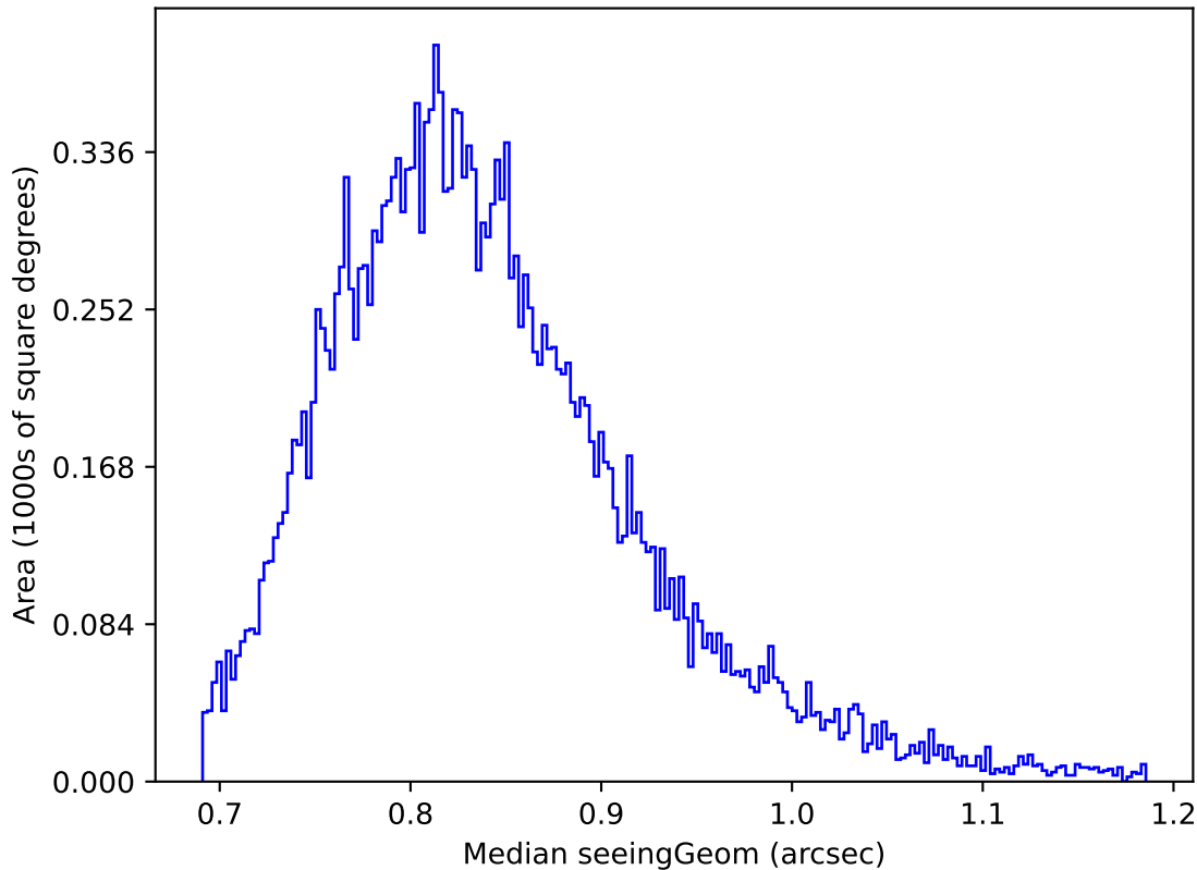
too_elab_r16_d2_gz_v3.4_10yrs Yr 1 y band: Median seeingGeom
