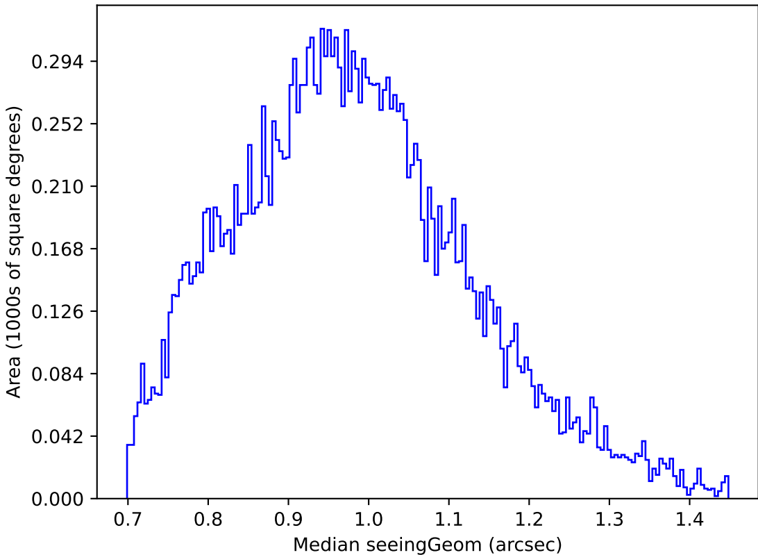
too_elab_r16_d2_gz_v3.4_10yrs Yr 1 u band: Median seeingGeom
