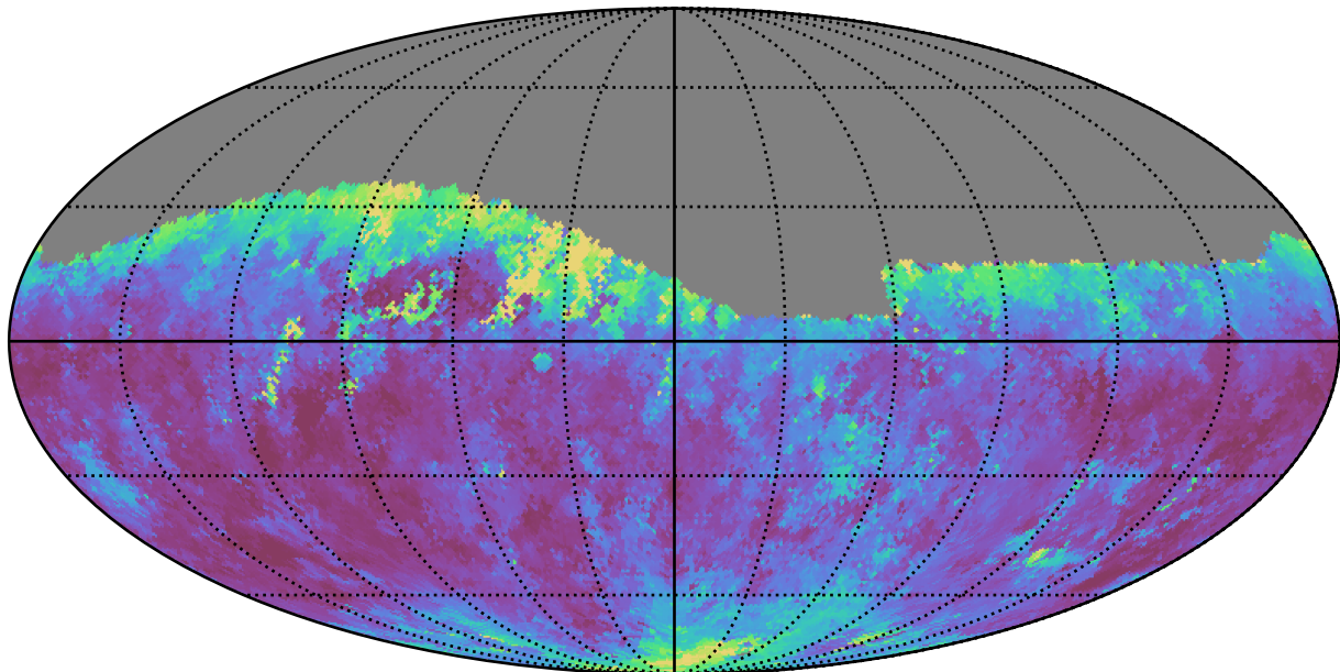
too_elab_r16_d2_gz_v3.4_10yrs Yr 1 r band: Median seeingGeom
