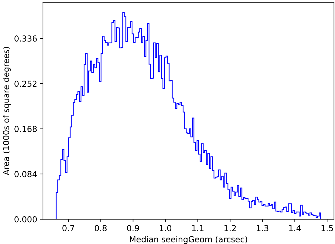
too_elab_r16_d2_gz_v3.4_10yrs Yr 1 g band: Median seeingGeom
