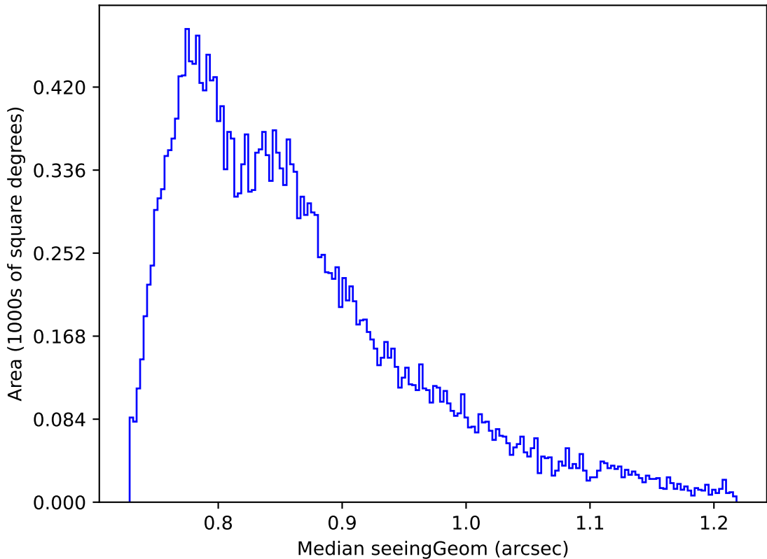
too_elab_r16_d2_gz_v3.4_10yrs Yr 1 all bands: Median seeingGeom
