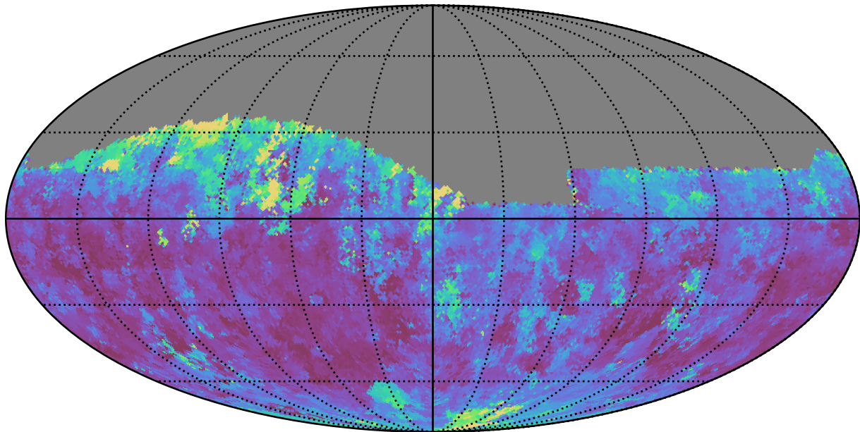
too_elab_r16_d2_gz_v3.4_10yrs Yr 1 z band: Median seeingEff
