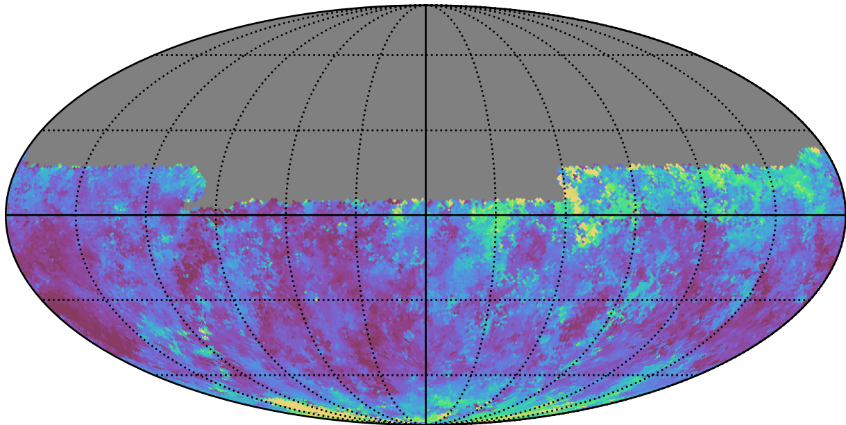
too_elab_r16_d2_gz_v3.4_10yrs Yr 1 y band: Median seeingEff
