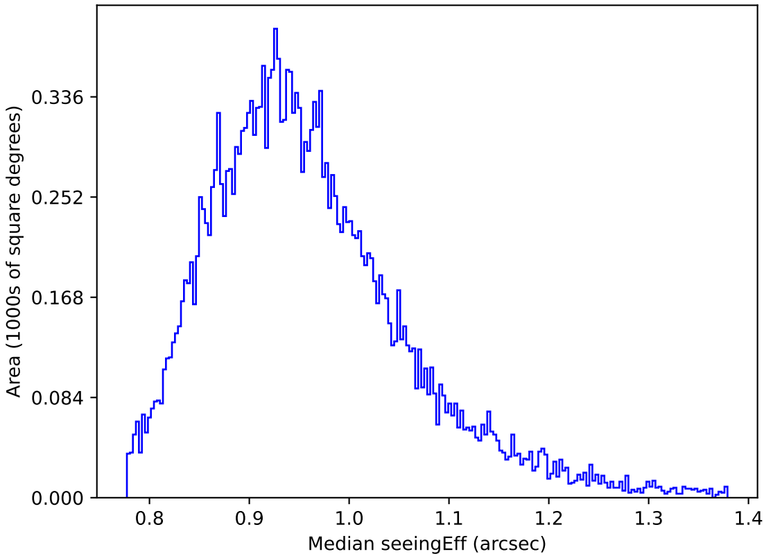
too_elab_r16_d2_gz_v3.4_10yrs Yr 1 y band: Median seeingEff
