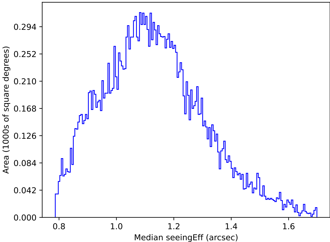
too_elab_r16_d2_gz_v3.4_10yrs Yr 1 u band: Median seeingEff
