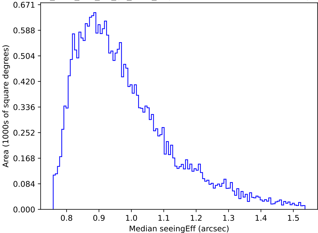
too_elab_r16_d2_gz_v3.4_10yrs Yr 1 r band: Median seeingEff
