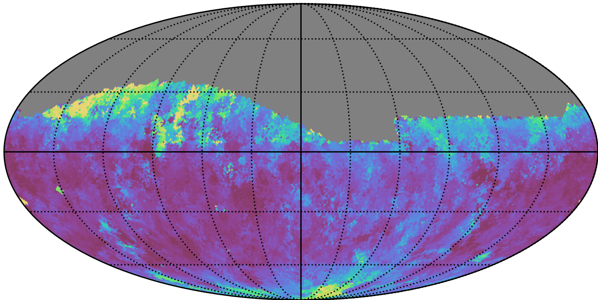
too_elab_r16_d2_gz_v3.4_10yrs Yr 1 i band: Median seeingEff
