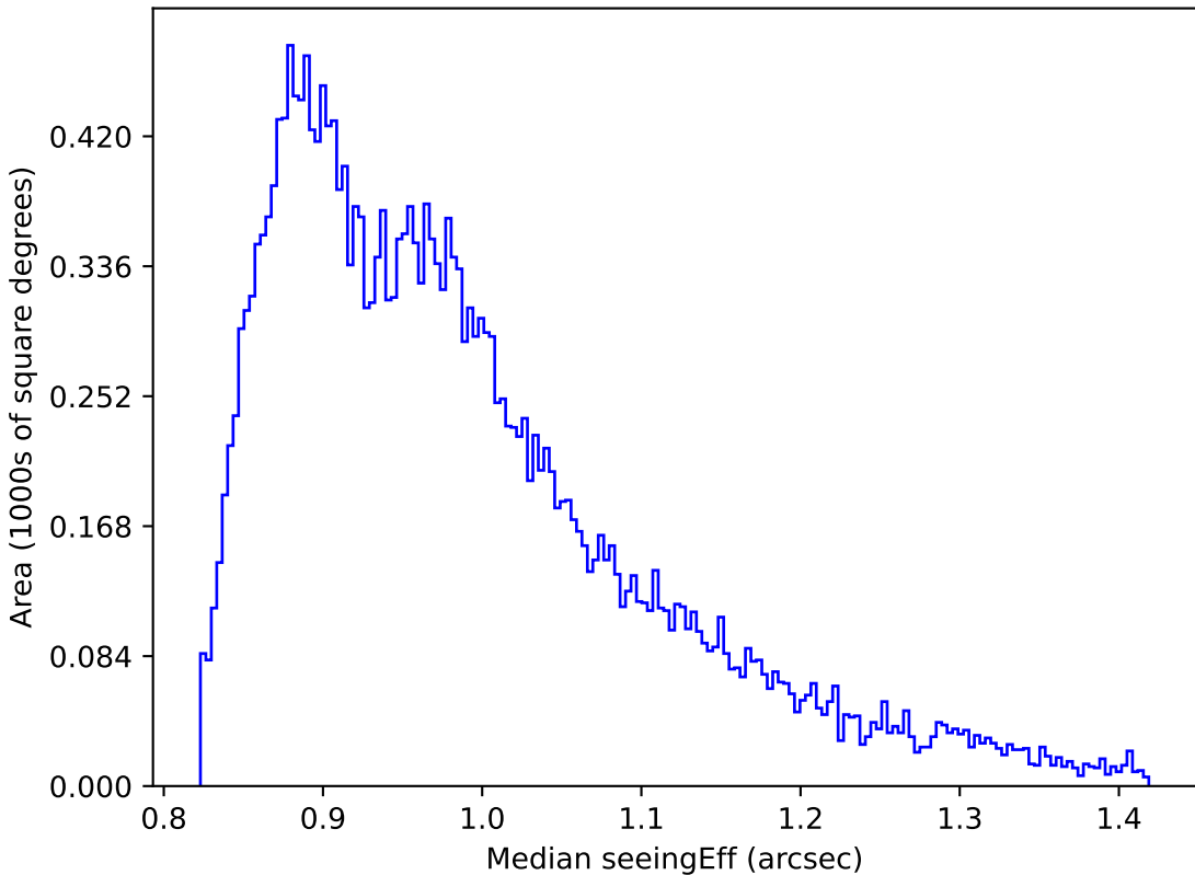
too_elab_r16_d2_gz_v3.4_10yrs Yr 1 all bands: Median seeingEff
