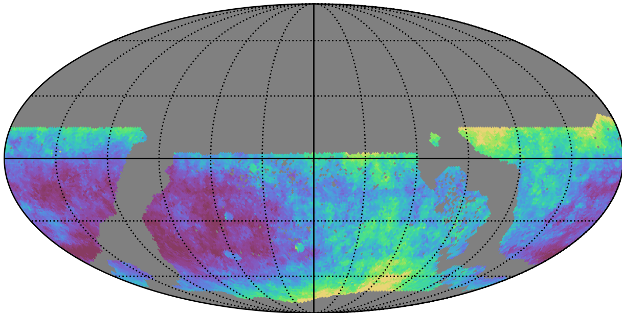
too_elab_r16_d2_gz_v3.4_10yrs WFD z band: Median seeingEff
