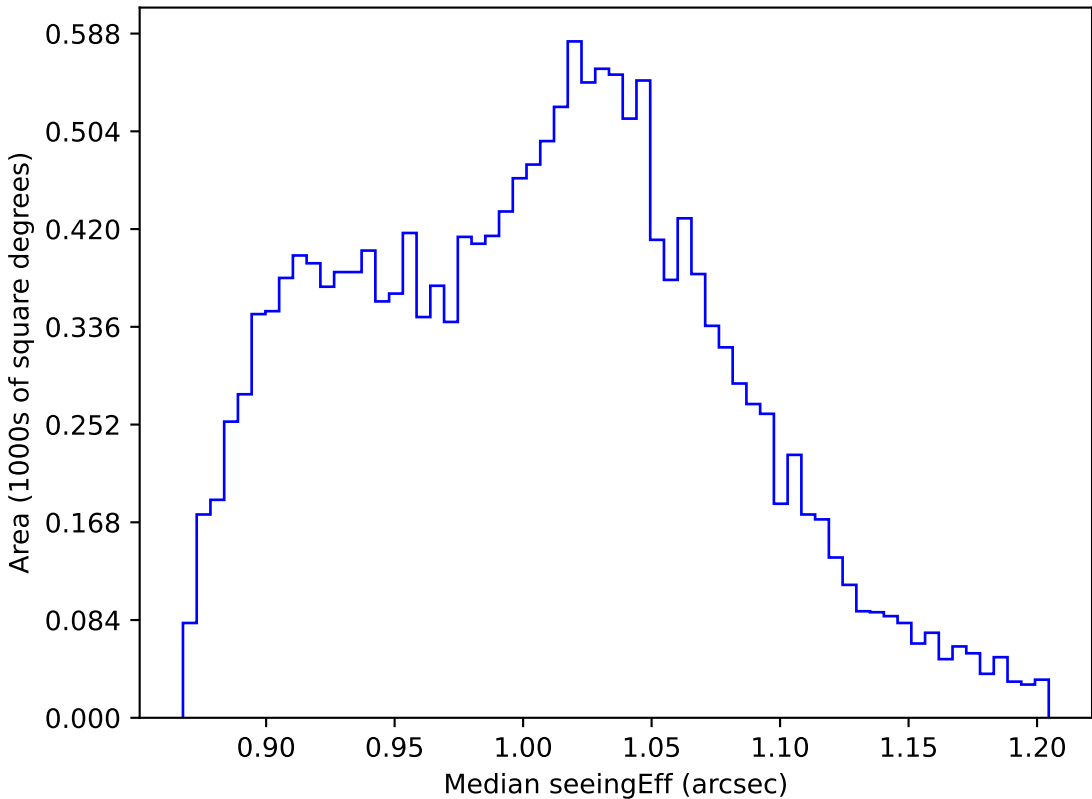
too_elab_r16_d2_gz_v3.4_10yrs WFD z band: Median seeingEff
