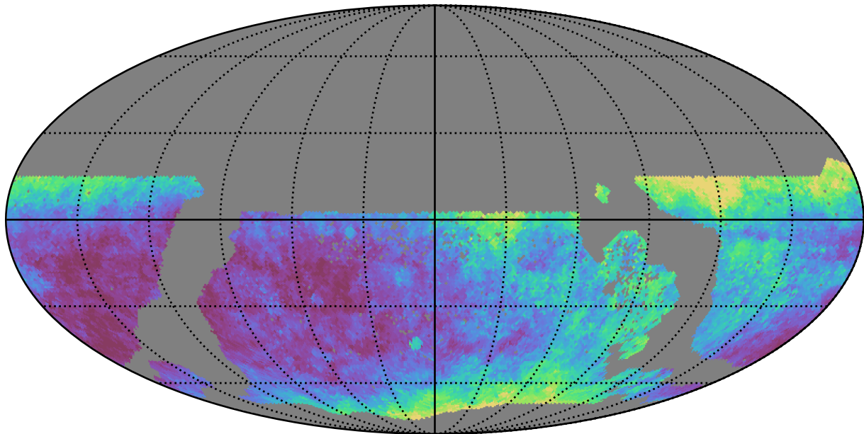
too_elab_r16_d2_gz_v3.4_10yrs WFD y band: Median seeingEff
