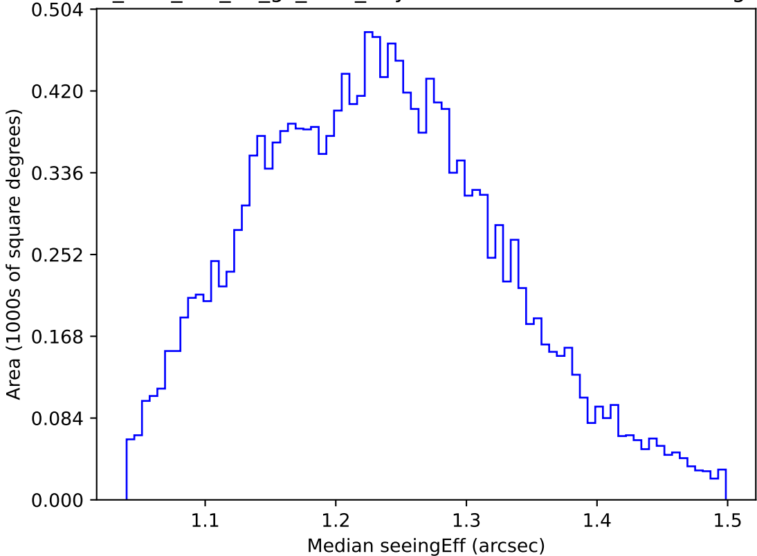
too_elab_r16_d2_gz_v3.4_10yrs WFD u band: Median seeingEff
