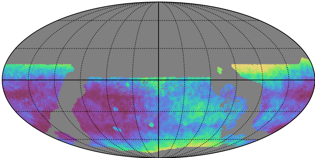
too_elab_r16_d2_gz_v3.4_10yrs WFD r band: Median seeingEff
