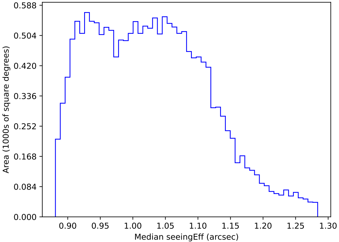
too_elab_r16_d2_gz_v3.4_10yrs WFD r band: Median seeingEff
