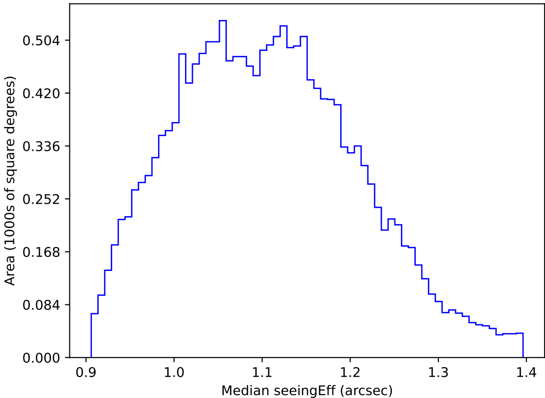
too_elab_r16_d2_gz_v3.4_10yrs WFD g band: Median seeingEff
