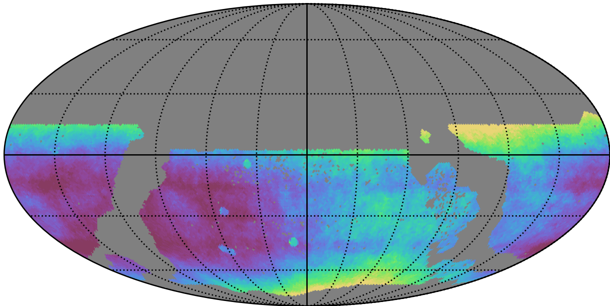
too_elab_r16_d2_gz_v3.4_10yrs WFD all bands: Median seeingEff
