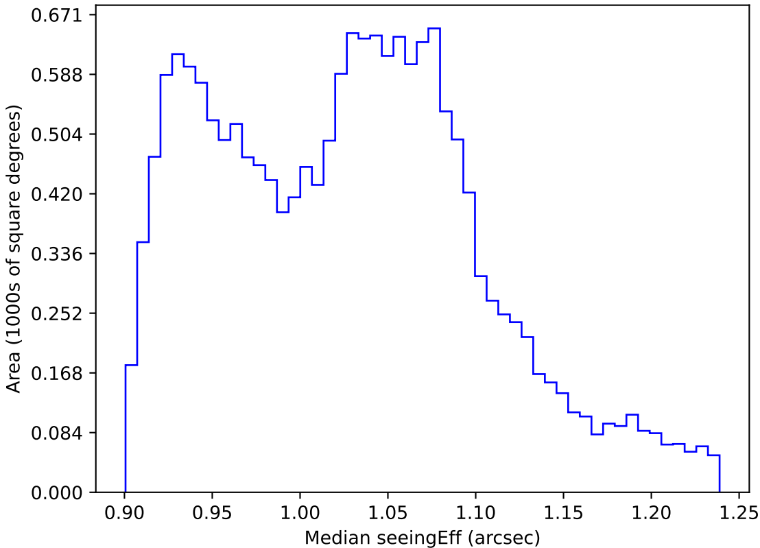
too_elab_r16_d2_gz_v3.4_10yrs WFD all bands: Median seeingEff
