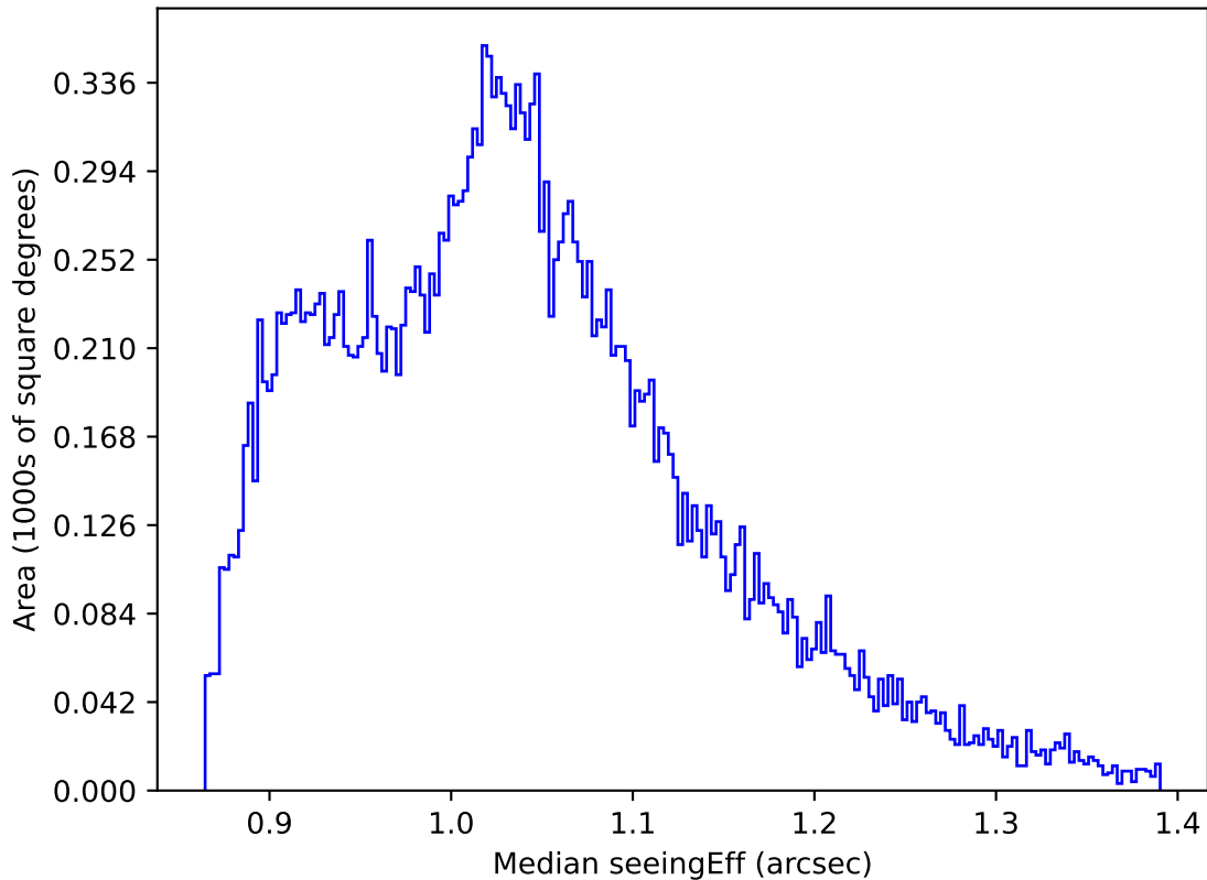
too_elab_r16_d2_gz_v3.4_10yrs All sky z band: Median seeingEff
