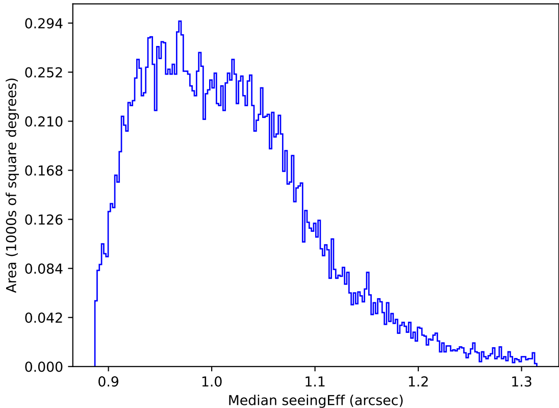
too_elab_r16_d2_gz_v3.4_10yrs All sky y band: Median seeingEff
