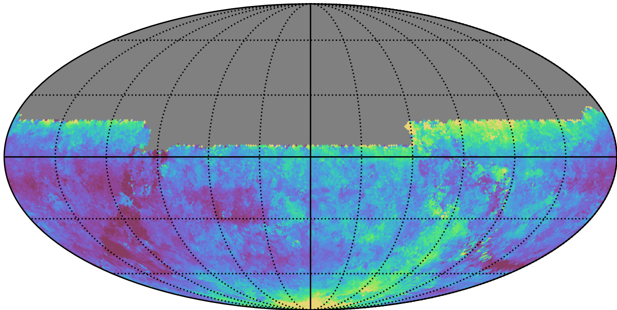
too_elab_r16_d2_gz_v3.4_10yrs All sky u band: Median seeingEff
